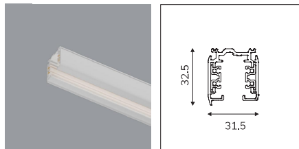
3 Circuit Track (Surface Mounted) 1M/1.5M/2M/3M Length
