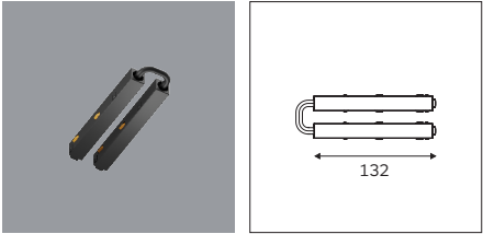
FLEXIBLE CONNECTOR
